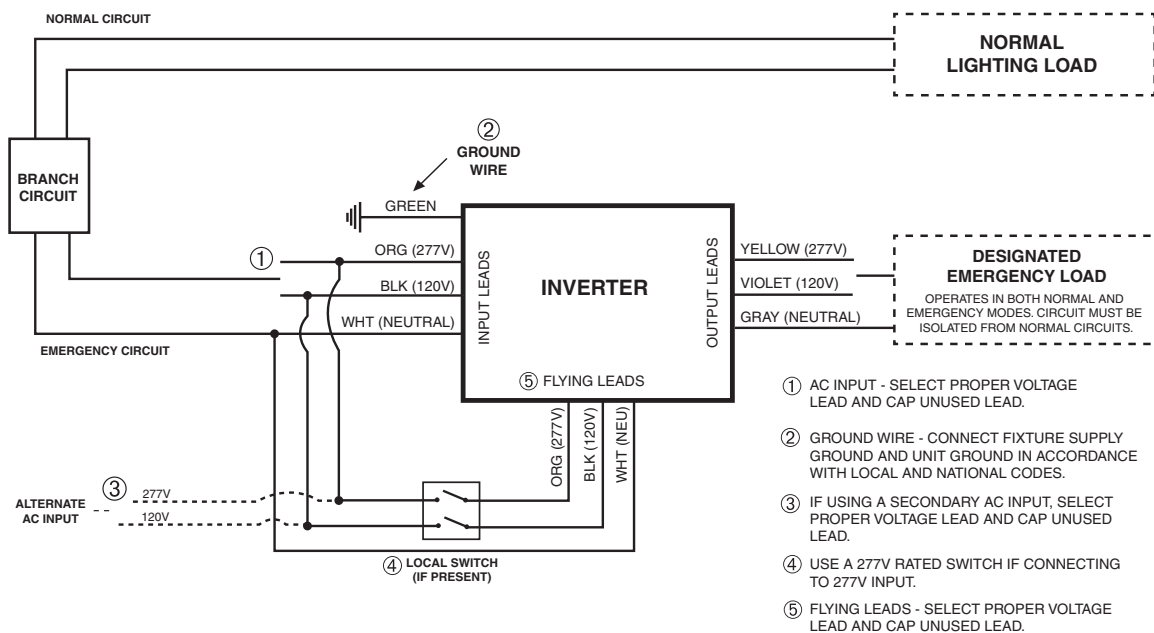
FIGURE 1 - IIS 125 WIRING CONNECTIONS
